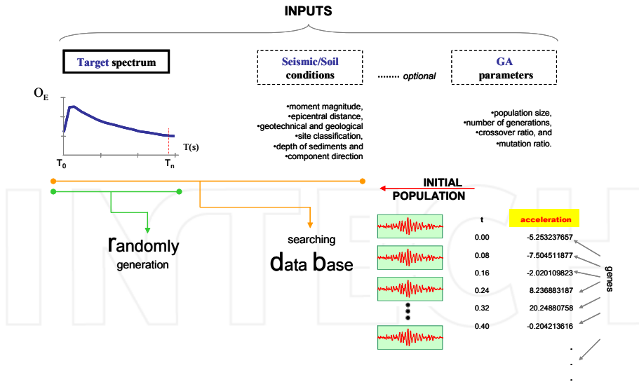
Figure 11. Genetic Generator: working phase diagram
