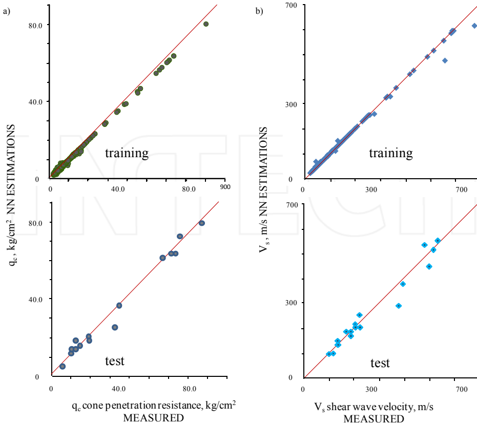
Figure 3. Neural estimations of mechanical and dynamic parameters
