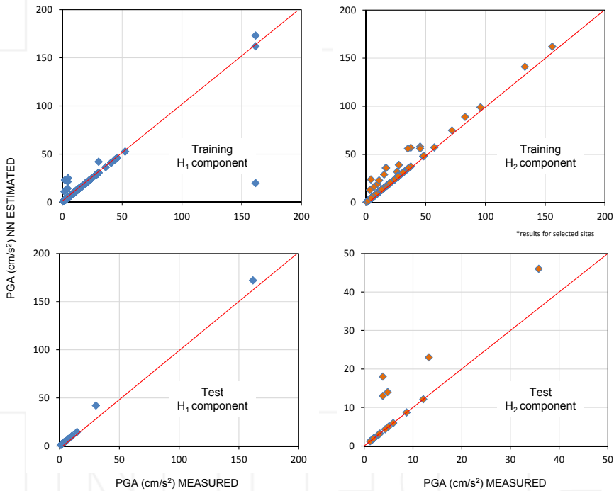
Figure 15. Neural estimations for PGA in Lake Zone sites
