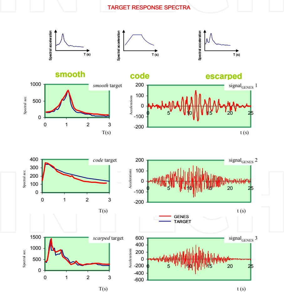
Figure 13. Some Generator results: accelerograms application
