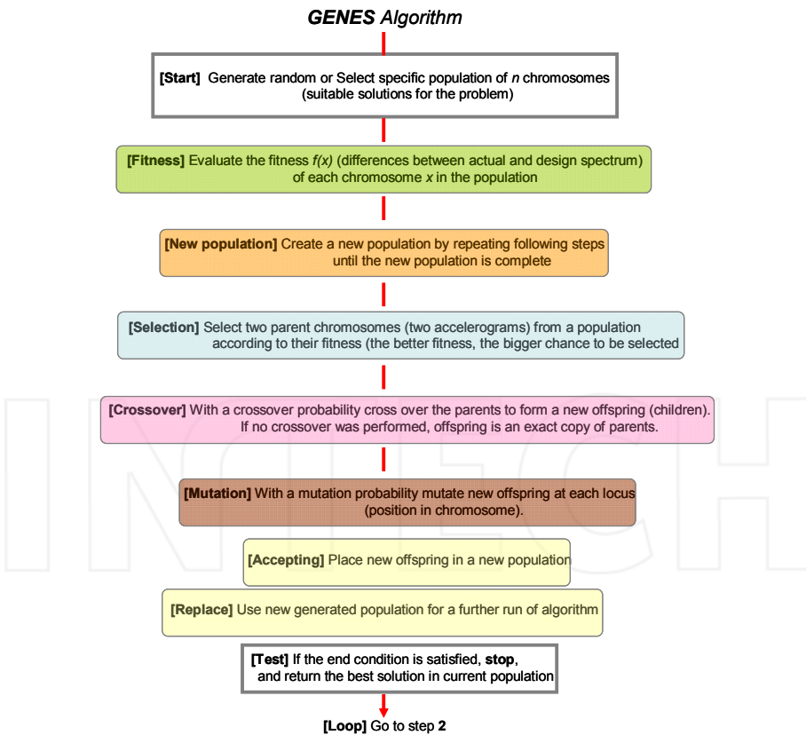
Figure 10. Genetic Generator: flow diagram
