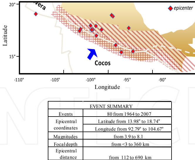
Figure 6. Earthquakes characteristics
