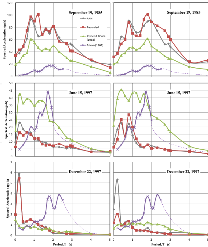
Figure 9. Response Spectra: NN-calculated vs traditional functions
