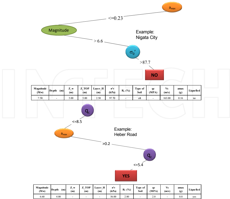
Figure 19. CT classification examples
