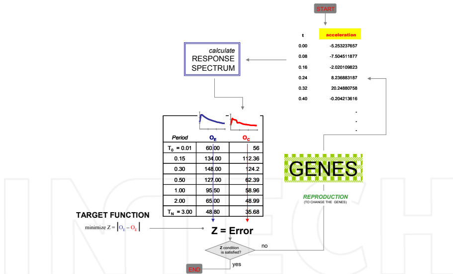
Figure 12. Iteration process of the Genetic Generator
