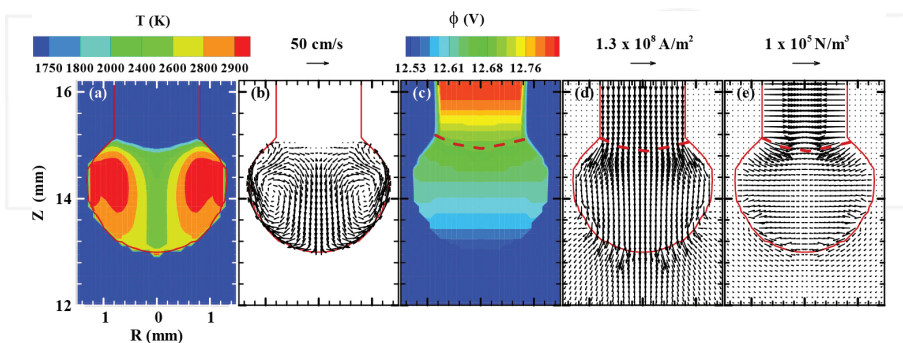
Figure 7. Distribution of physical variables within the droplet at t = 100 ms. (a) Temperature, (b) velocity, (c) electrical potential, (d) current density, and (e) electromagnetic force.
