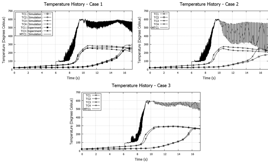
Figure 9. Temperature history results for the three cases.
