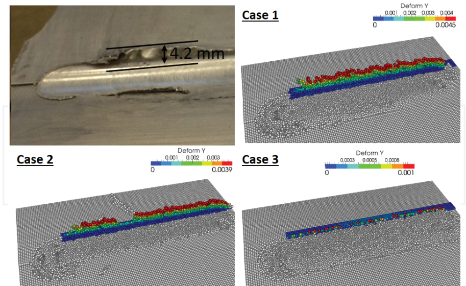
Figure 11. Flash height comparison at the end of advancing phase.
