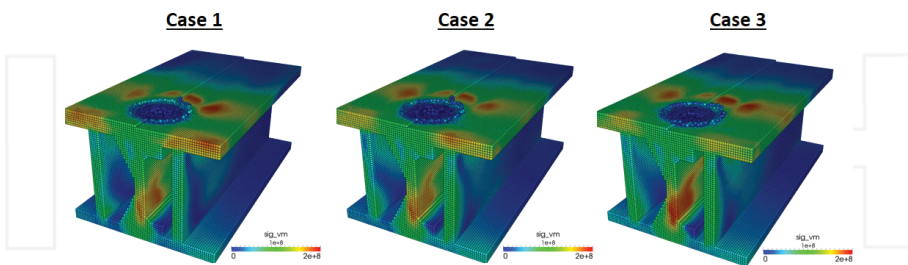
Figure 13. Stress state at the end of plunge phase.
