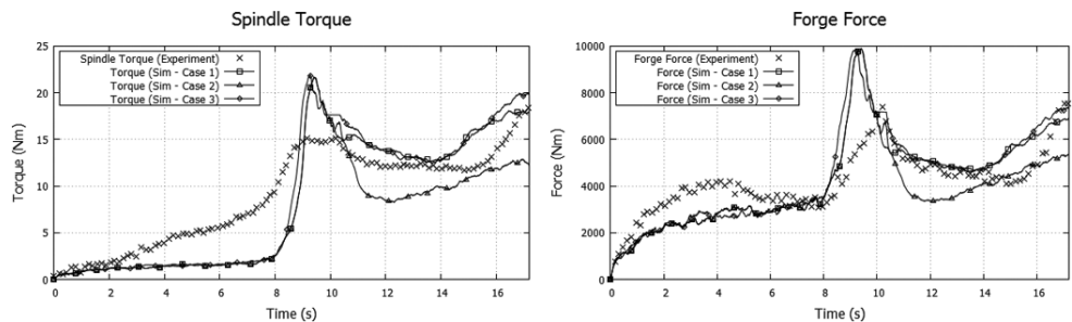
Figure 10. Spindle torque and forge-force comparison.
