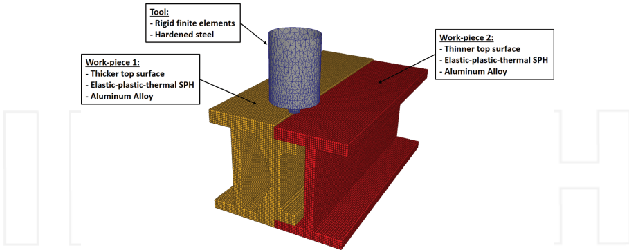
Figure 6. FSW joint simulation model.
