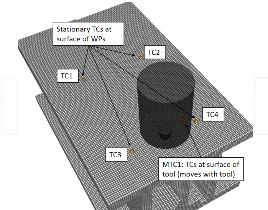
Figure 8. Temperature measurement points in the simulation model.
