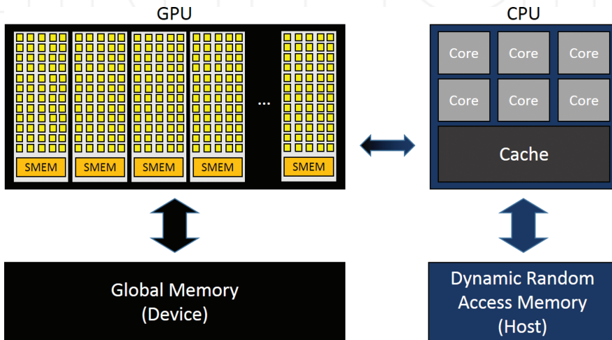
Figure 4. GPU architecture (adapted from NVIDIA [32] and Ruetsch and Fatica [33]).
