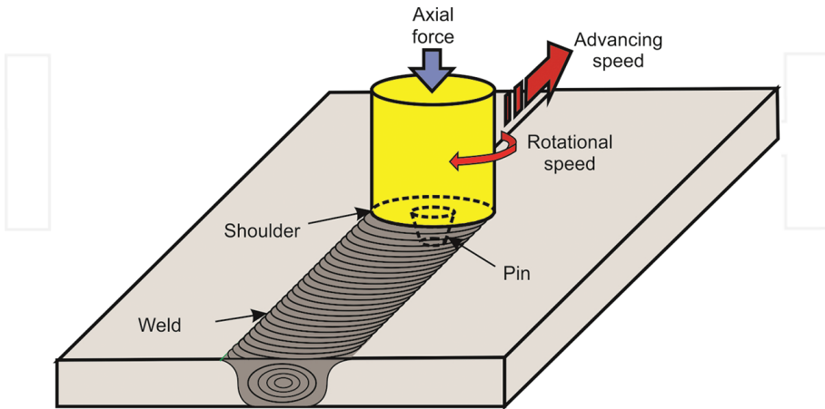
Figure 1. Friction stir-welding process.
