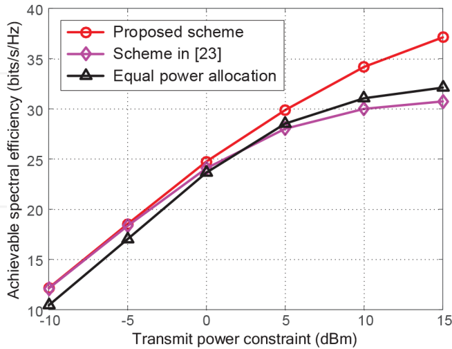
Figure 6. Comparison of achievable SE by different schemes.
