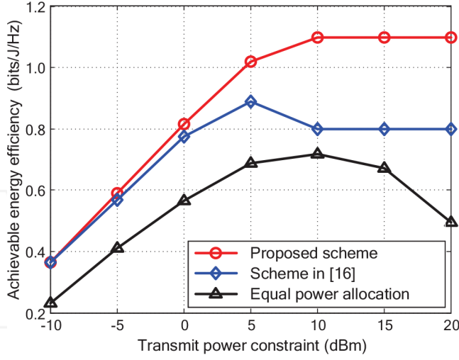
Figure 5. Comparison of achievable EE by different schemes.
