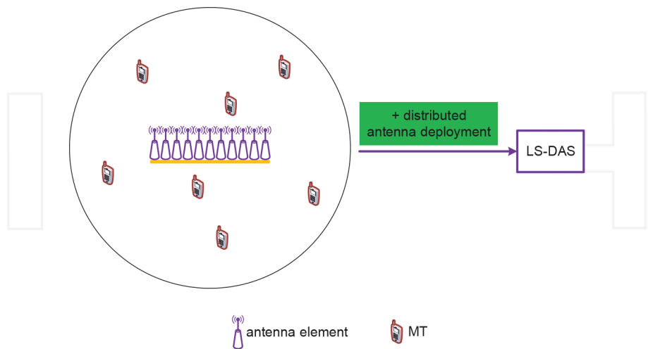
Figure 2. Illustration of a traditional large-scale MIMO system.
