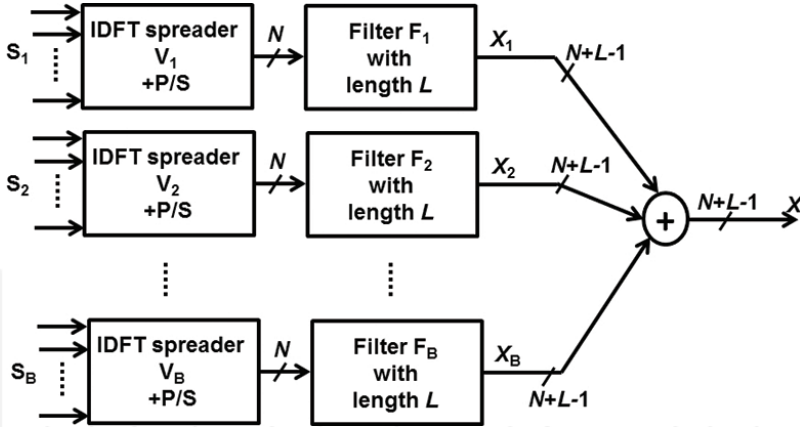
Figure 5. UFMC transmitter.
