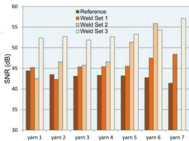
Figure 16. Comparison of SNR values of welded samples (weld set 1: T = 350^{\circ}\text{C} , v = 2.5 \text{ m/min} , p = 6.5 \text{ bar} ; weld set 2: T = 450^{\circ}\text{C} , v = 2.5 \text{ m/min} , p = 6.5 \text{ bar} ; weld set 3: T = 350^{\circ}\text{C} , v = 1.5 \text{ m/min} , p = 6.5 \text{ bar} ).
