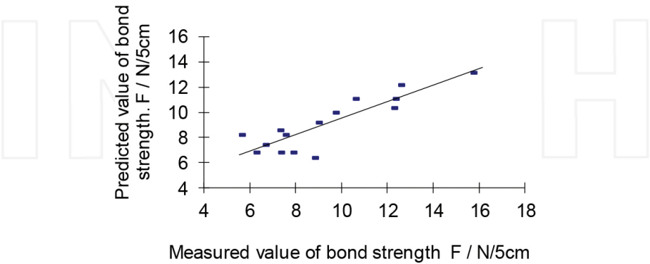
Figure 13. Correlation between the measured and predicted values of bond strength.
