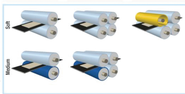
Figure 6. FLEXO Double Pressure System DXT 1400L/1600 CFC [14].
