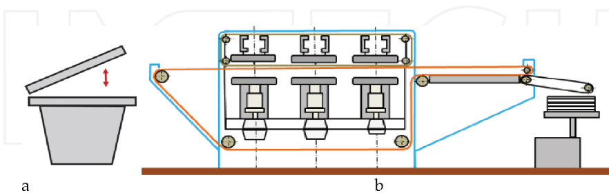
Figure 4. Flat-bed press (a) and continuous fusing machine (b).
