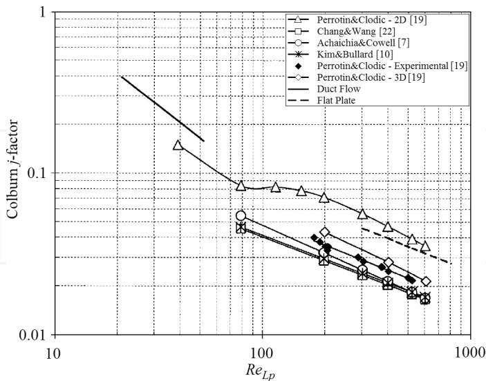
Figure 13. Comparison of computed and measured j -factor [19].
