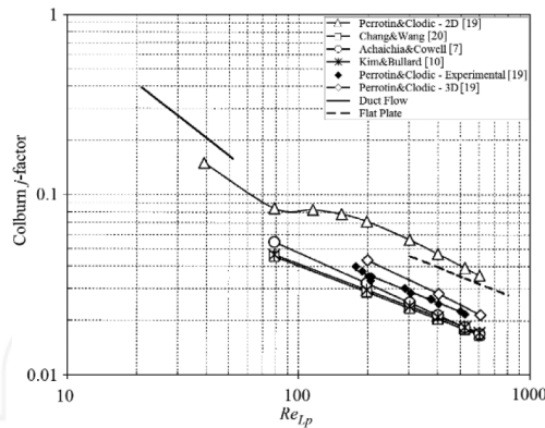
Figure 14. Comparison of computed and measured f -factor [19].
