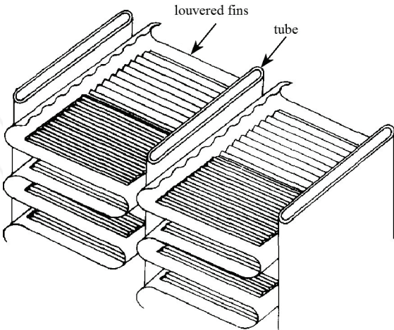
Figure 2. Typical structure of a louver fin geometry [4].
