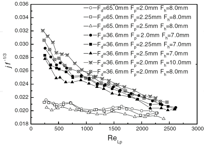
Figure 22. The variation of j/f^{1/3} [15].
