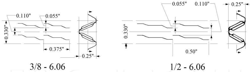
Figure 3. Terminology of the louvered fin [2].
