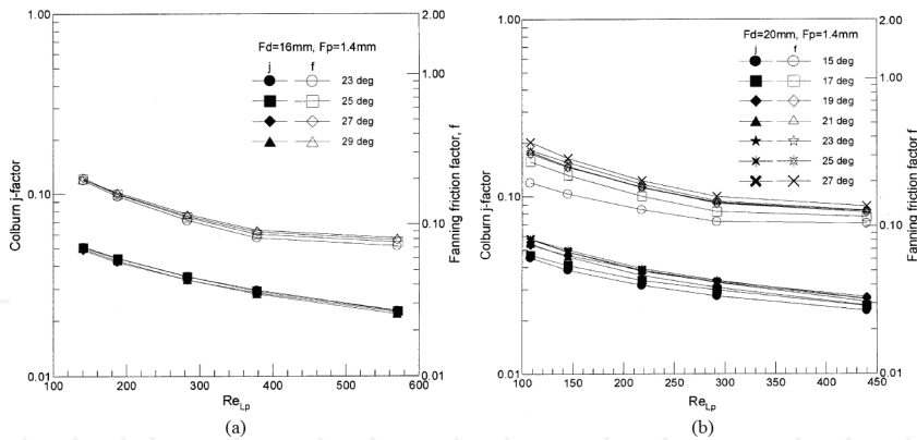
Figure 20. Variations of j -factor and f -factor with respect to the louver angle and Reynolds number for (a) F_d = 16 mm and (b) F_d = 20 mm [10].
