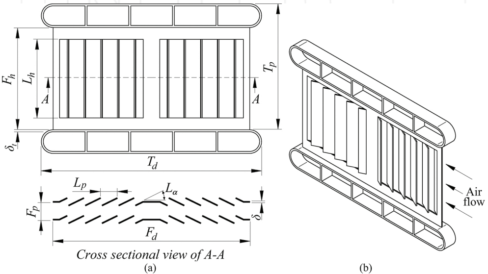
Figure 4. Terminology of the louvered fin [6].
