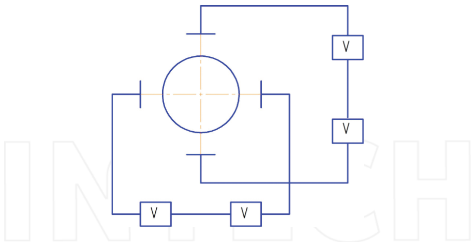
Figure 6. The electrostatic support.
