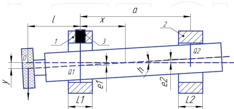
Figure 5. Hybrid gas-magnetic shaft suspension of high-speed spindle: 1—front gas-magnetic bearing; 2—rear gas-static bearing; 3—electromagnet.
