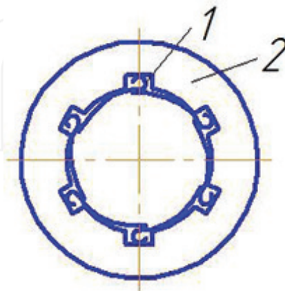
Figure 1. Aerodynamic bearing: 1—trunnion; 2—foil.
