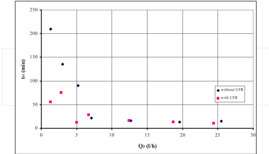
Figure 5. Stabilisation time of water flow in the installation t_{st} in the function of flow Q_3 .
