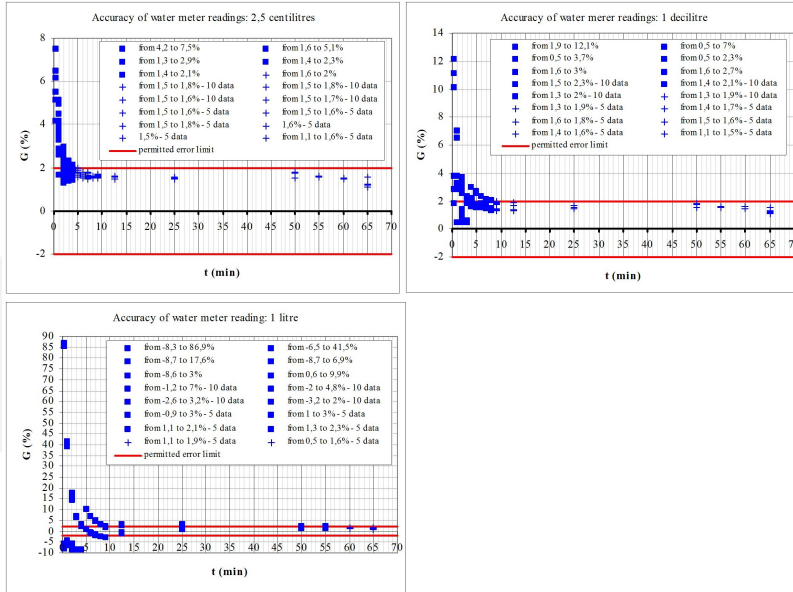
Figure 11. Error in water meter measuring at Q_c flow during water flow shorter than the time for which the meter was calibrated (12.5 min.) in the function of water meter reading accuracy.
