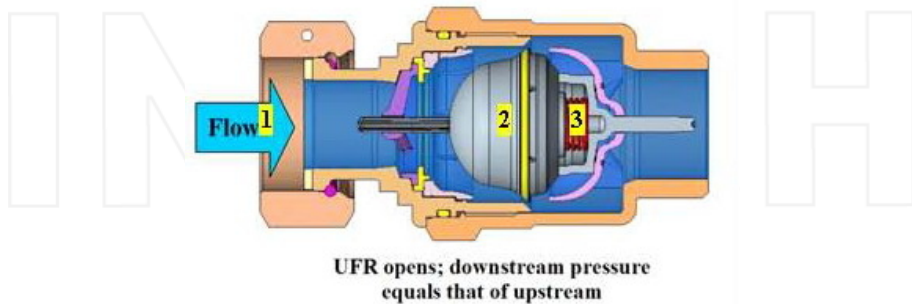
Figure 1. Structure of the UFR- manufactured by A.R.I. from Jerusalem (Israel) [4] 1 - flow direction, 2 - UFR plug, 3 - UFR spring.
