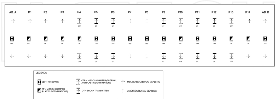
Figure 6. Restraint diagram.
