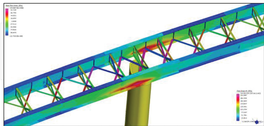
Figure 16. Stresses on the steel elements.
