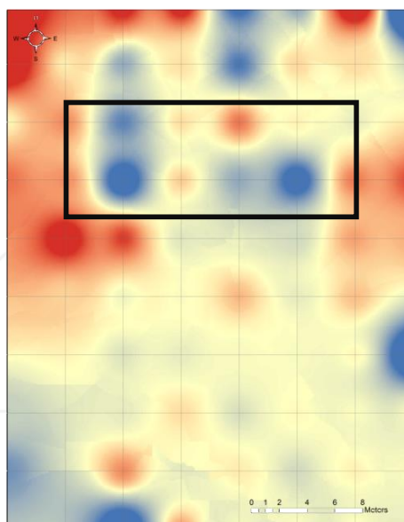
Figure 25. Difference values as calculated for ARVI index
