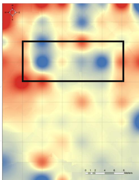
Figure 20. Difference values as calculated for MSAVI index
