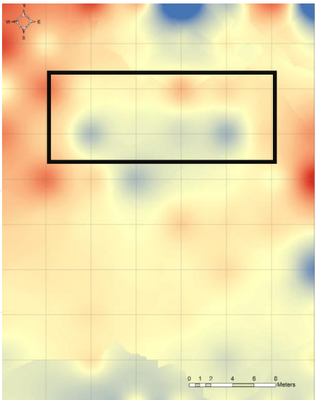
Figure 23. Difference values as calculated for GEMI index
