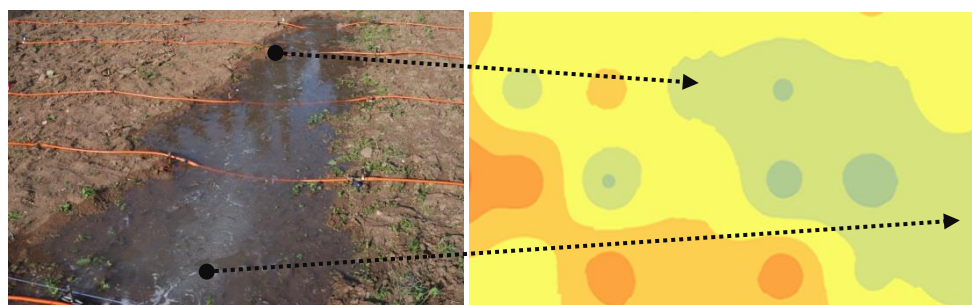
Figure 8. Detail of Figure 4. The lowest temperature values were recorded in the area where the leakage was still ongoing. The temperature map was able to draw with relative high precision the problematic area
