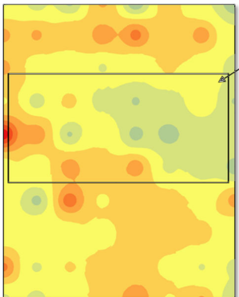
Figure 7. Ground temperature over the area of interest as recorded from the digital laser thermometer, during the leakage event. Rectangle indicates the location of the buried pipeline. Blue values indicates temperatures 14-16°C, 24-26°C are shown in yellow while orange colour highlight values from 34-36°C
