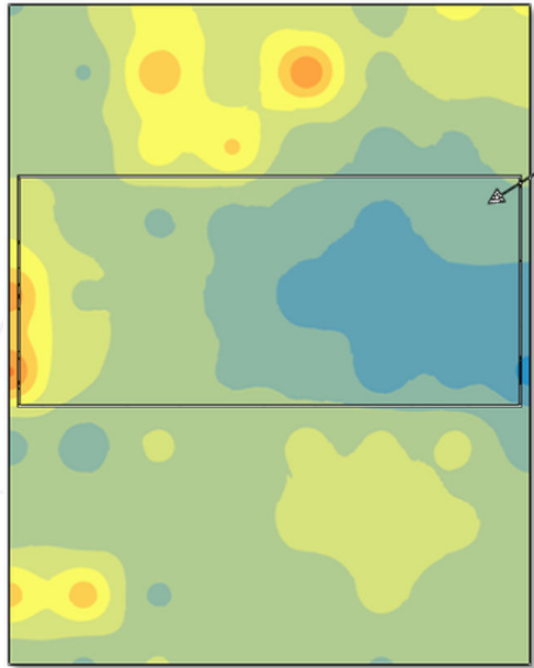
Figure 9. Ground temperature over the area of interest as recorded from the digital laser thermometer, during the leakage event. Rectangle indicates the location of the buried pipeline. Blue values indicates temperatures 14-16°C, 24-26°C are shown in yellow while orange colour highlight values from 34-36°C
