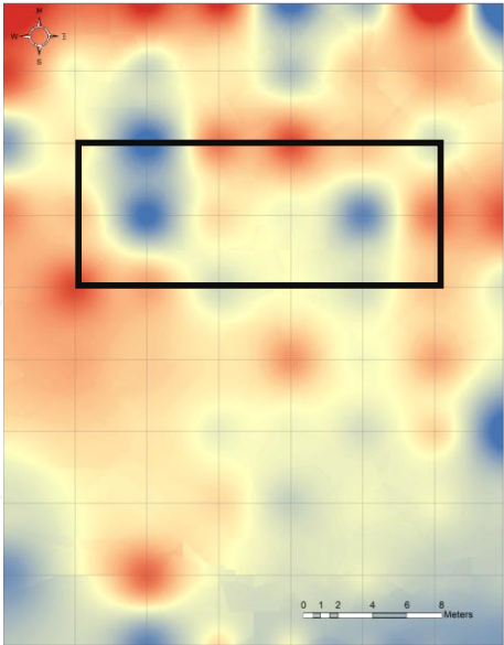
Figure 22. Difference values as calculated for GNDVI index
