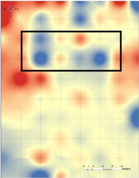
Figure 15. Difference values as calculated for SARVI index
