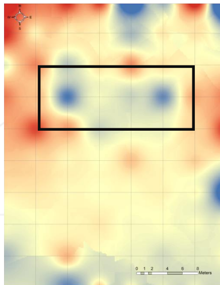
Figure 13. Difference values as calculated for SRxNDVI index
