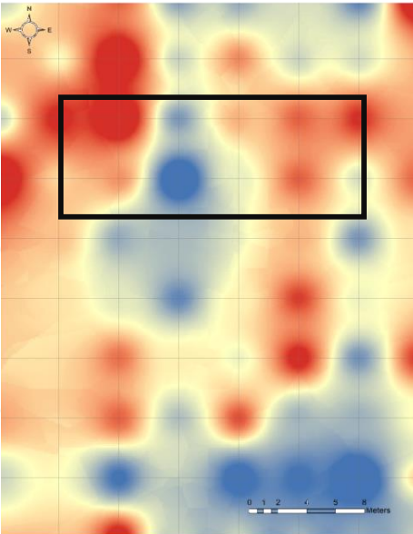
Figure 19. Difference values as calculated for MSR index
