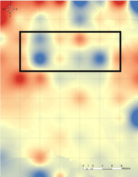
Figure 14. Difference values as calculated for SR index
