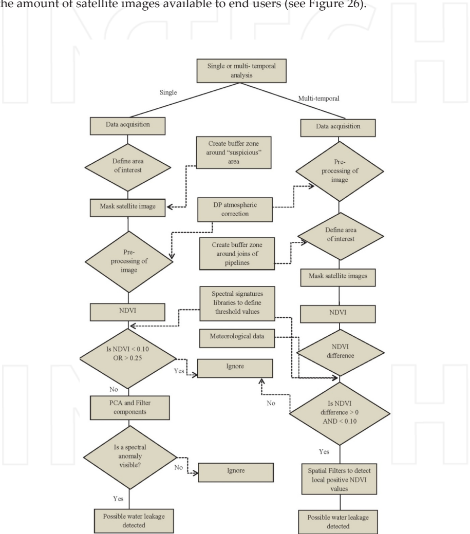
Figure 26. Methodology followed for the early warning system (Agapiou et al. 2014).
