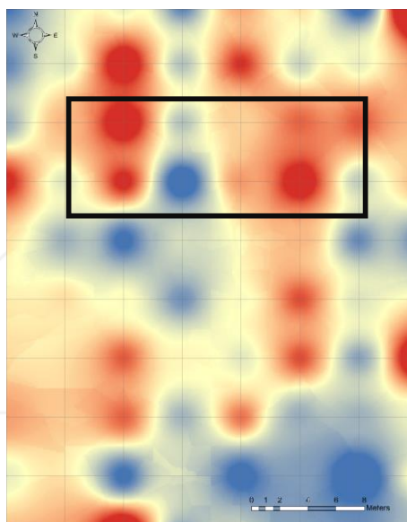
Figure 21. Difference values as calculated for IRG index
