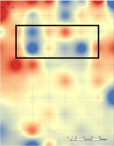
Figure 18. Difference values as calculated for NDVI index
