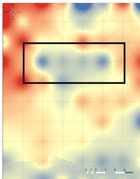
Figure 24. Difference values as calculated for DVI index
