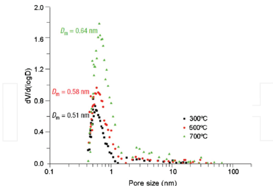
Figure 3. Differential pore size distribution for CDC-synthesized membrane at varying chlorination temperatures measured by methyl chloride adsorption (reprinted with permission from Gogotsi et al. [19]).
