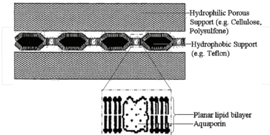
Figure 11: Schematic cross section of aquaporin-embedded membrane [72].
