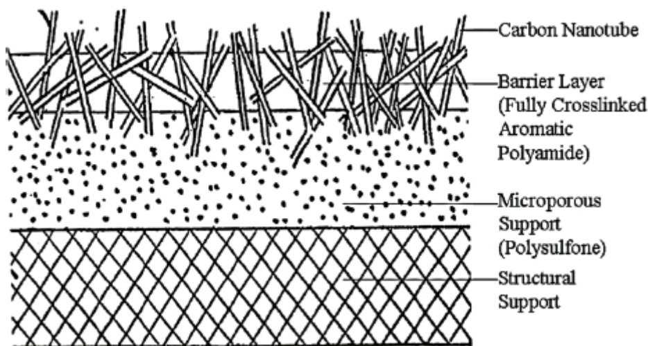
Figure 8. Schematic cross-section of CNTs-embedded TFC membrane [64].
