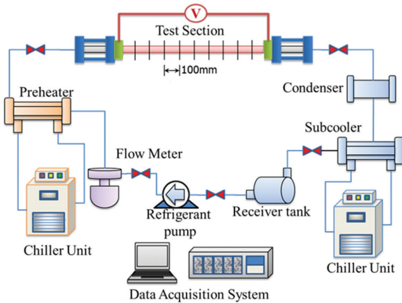
Figure 1. The experimental apparatus: (a) copper tube and (b) stainless tube.
