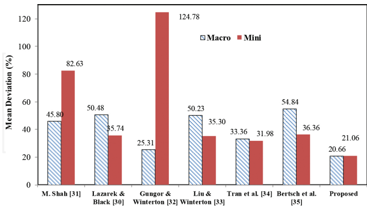
Figure 13. Summary of mean deviation.
