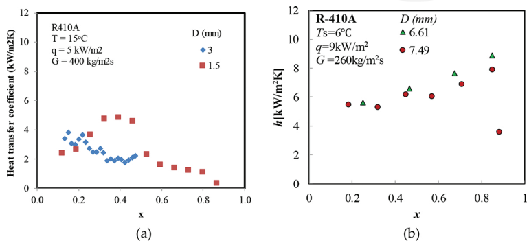
Figure 9. The effect of inner diameter on heat transfer coefficient of R410A : (a) Di = 1.5 & 3.0 mm; (b) Di = 6.61 & 7.49 mm.
