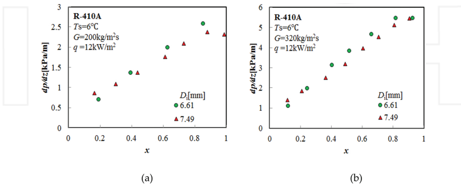
Figure 4. The effect of inner tube diameter on pressure drop of R410A: (a) G = 200 kg/m 2 s; (b) G = 320 kg/m 2 s.
