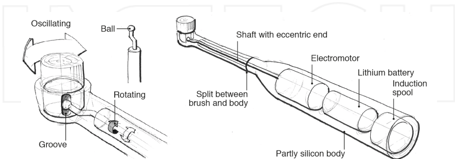
Figure 9. Sketches of the redesign - in this case the working principle is changed.
