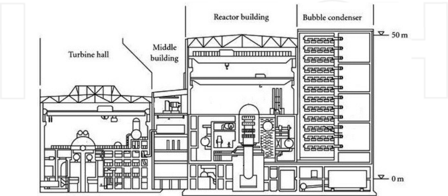
Figure 1. Section plane of the containment with reactor VVER440/213.
