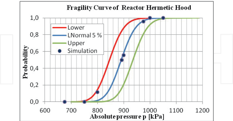
Figure 21. Fragility curves of the reactor-protective hood determined analytically for normal distribution with 5% envelope.
