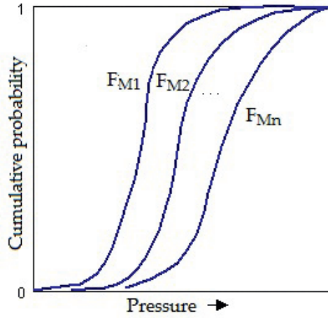
Figure 11. Family of fragility curves showing modelling uncertainty.
