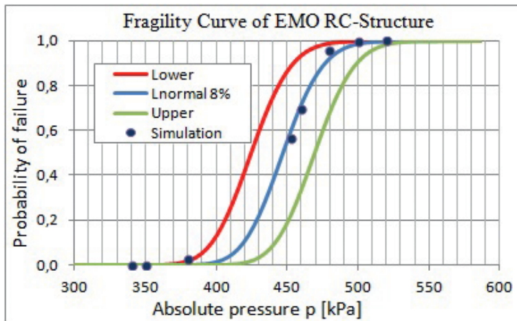
Figure 16. Fragility curve of failure pressure in the critical area of the hermetic zone under the accidental internal temperature T_i = 150^\circ\text{C} and external temperature T_e = -28^\circ\text{C} .
