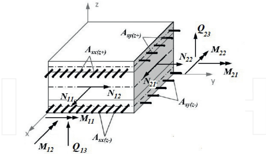
Figure 8. SHELL181-layered element with smeared reinforcements.
