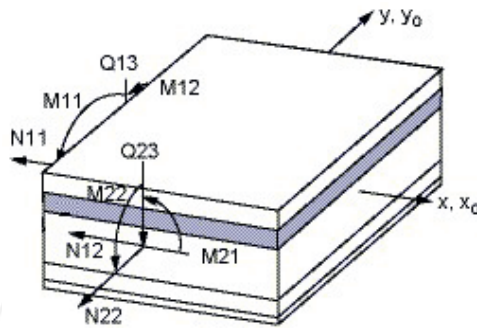
Figure 5. SHELL181-layered element with smeared reinforcements [26].
