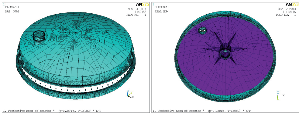
Figure 18. FEM model (RCOV) of the reactor-protective hood.
