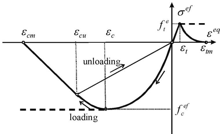
Figure 6. The concrete stress-strain diagram.
