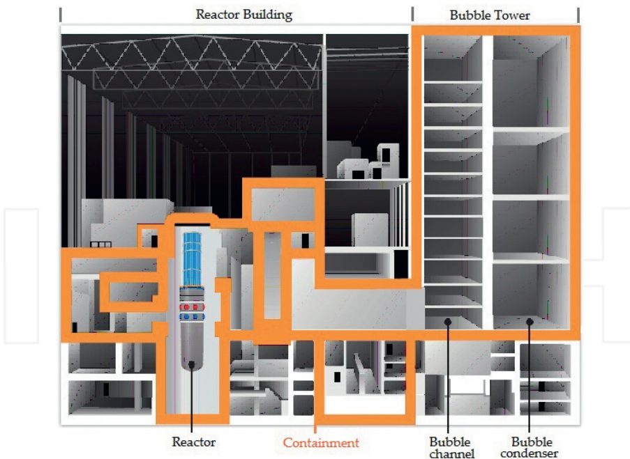
Figure 12. Section plane of the condenser containment.
