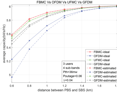
Figure 12. The relationship between distance and average capacity.
