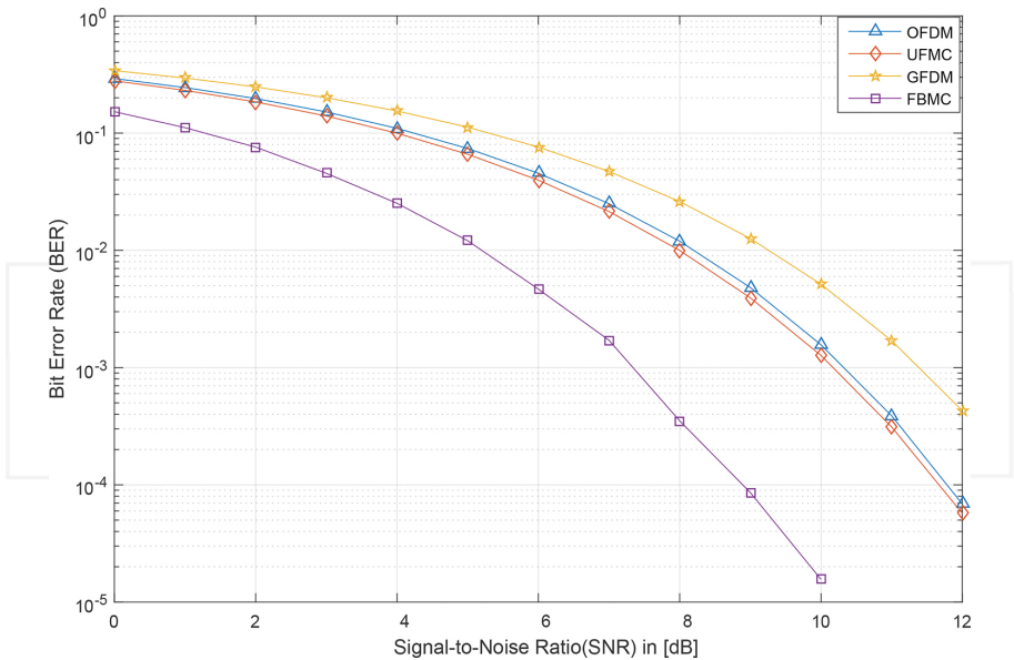
Figure 1. BER vs. SNR levels for FBMC-, OFDM-, GFDM-, and UFMC-based systems.
