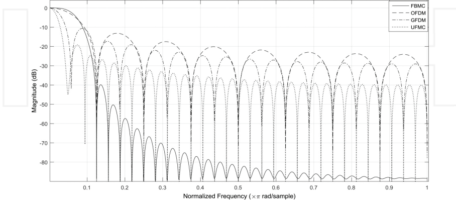
Figure 2. Frequency responses of prototype filters for FBMC, OFDM, GFDm, and UFMc.
