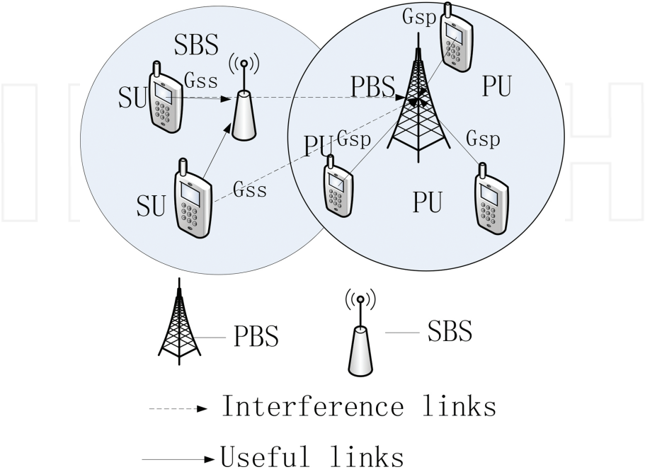
Figure 3. The system model of single CR cell including multiple users, the solid lines with arrow stand for the links producing the capacity, the dash lines with arrow stand for the interference links.
