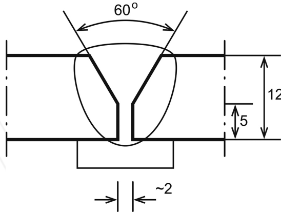
Figure 5. Scheme of the welded joint with technology chamfering.
