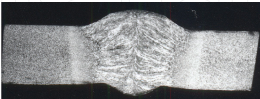
Figure 22. Cross-section of a welded joint: sample taken for metallographic analysis, magnification 2×.
