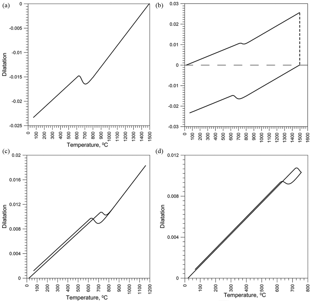
Figure 21. Dilatometric curves for selected points of cross-section.
