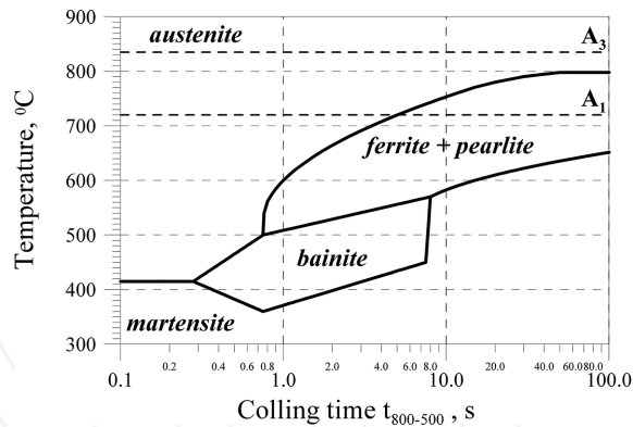
Figure 10. TTT-welding diagram for S235 steel.
