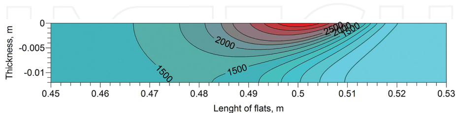
Figure 6. Temperature distribution (°C) on the surface of flats at time t = 102 s from beginning of welding.
