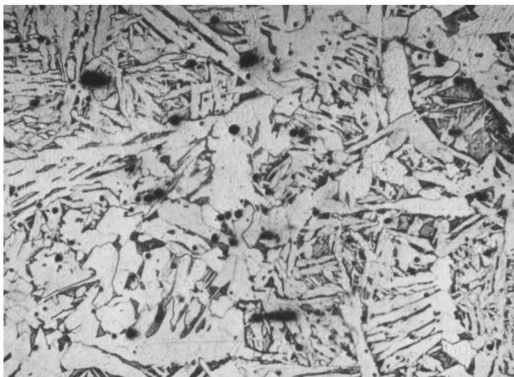
Figure 26. Heat affected zone, Nital Etch, magnification 250 \times , ferritic-pearlitic structure.
