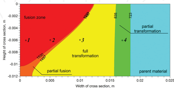
Figure 9. Heat-affected zones (HAZ) with selected points.
