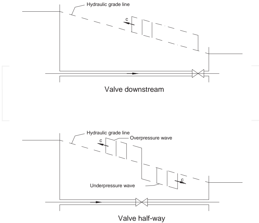
Figure 5. Pressure wave propagation following valve closure
