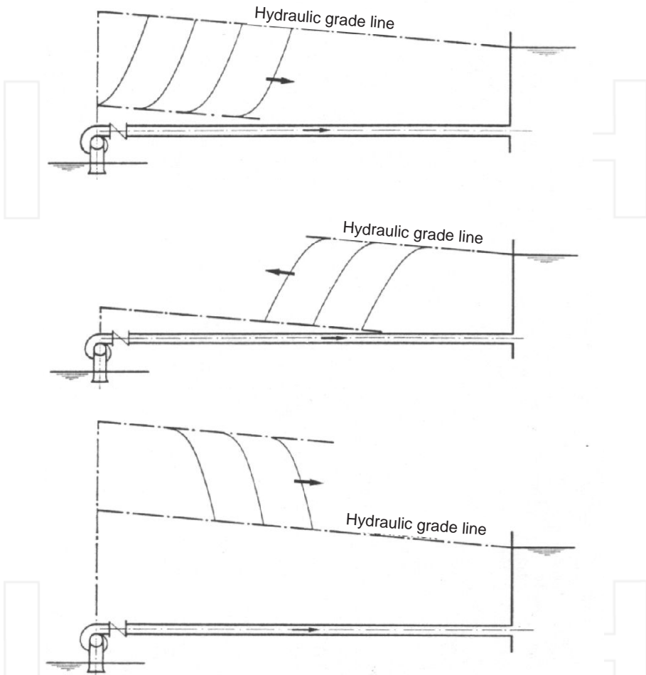
Figure 4. Pressure wave propagation following a pump trip
