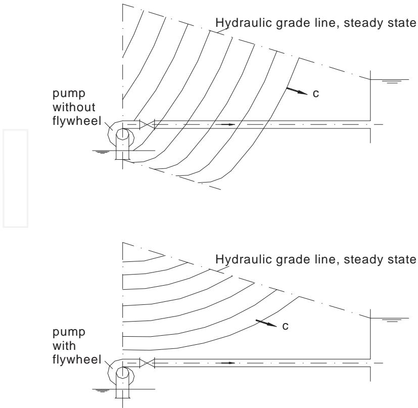
Figure 9. Effect of flywheel on transient pressure after power failure in the pumping station
