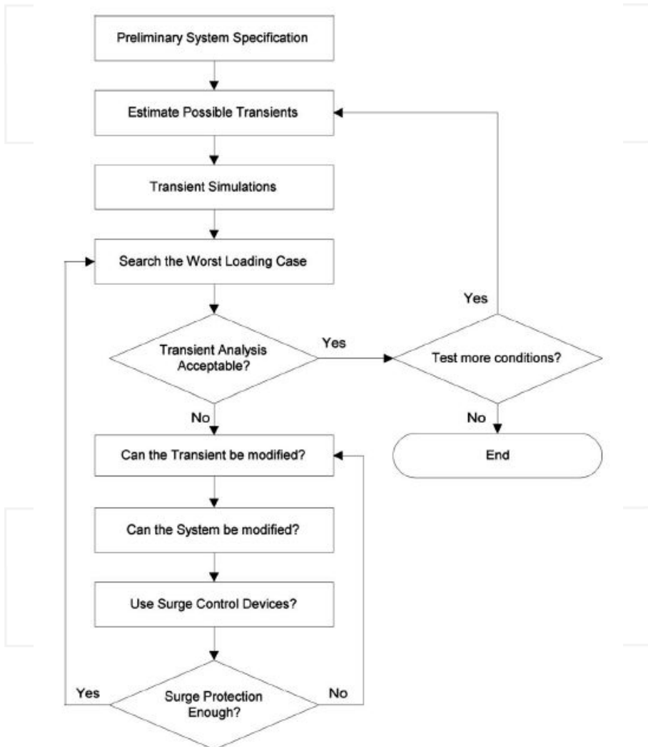
Figure 1. Pressure Transient design (Jung and Karney 2009).
