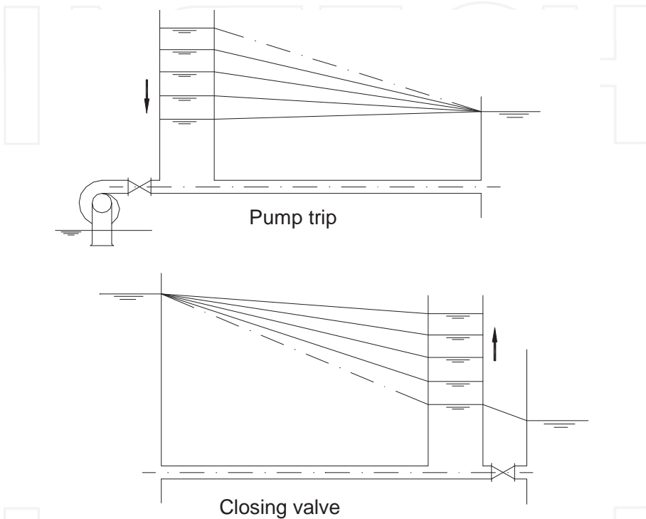
Figure 8. Surge tower near pumping station or valve station.
